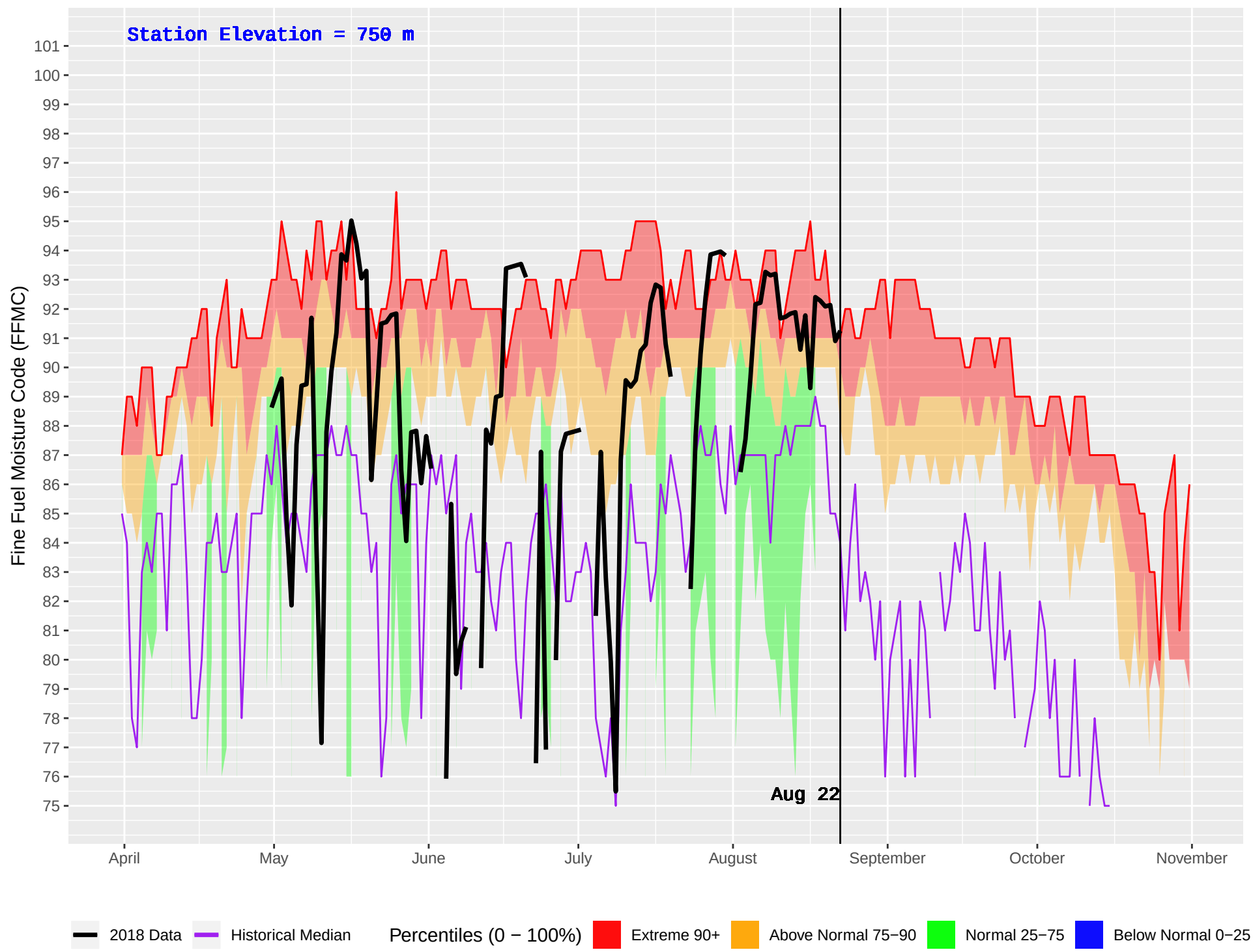
FORT ST JAMES (146) : Historical (1979–2016) and Current (2018) Daily Fine Fuel Moisture Code (FFMC)
